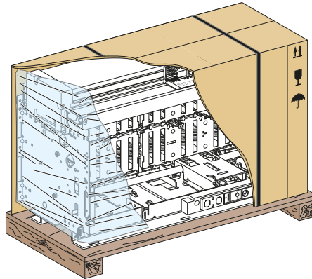
MTZ3 3P/4P
