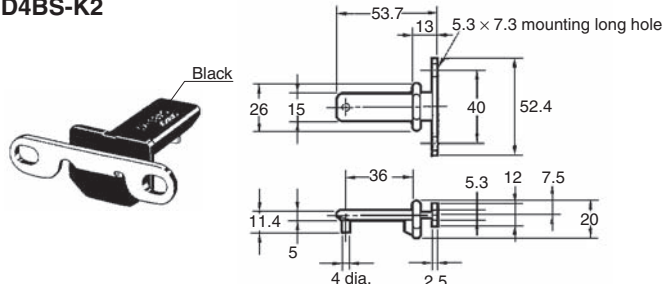
D4BS-K2
