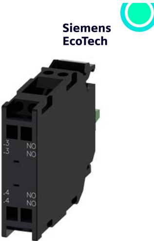
Contact module with 2 contact elements, 2 NO, spring-type terminal, for front plate mounting
