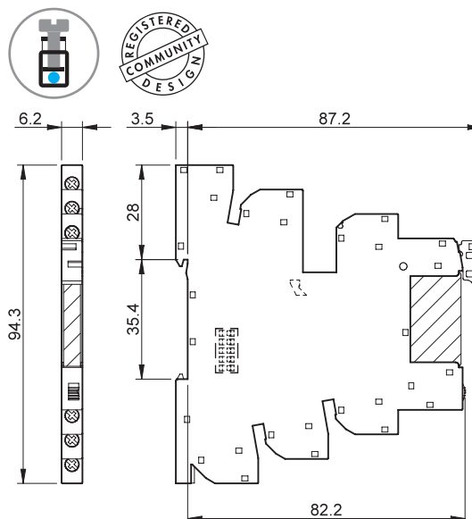
Types 39.80/39.81 Kooiklemmen
