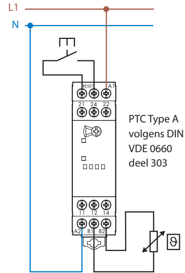
Type 70.92
