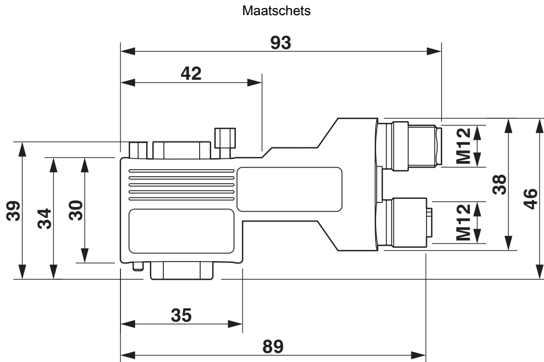
Maatschets SUBCON-PLUS...90X...M12, lange 90°-variant
