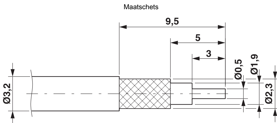
D-SUB-coaxcontact, bus
