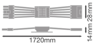
LN INV 1200 THROUGHWIRING KIT
