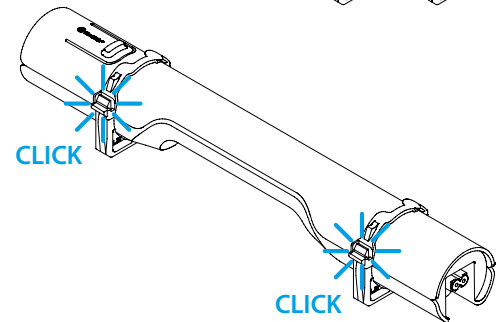
Plastic fixing ring Type 07L.22 (not included in the packaging)
