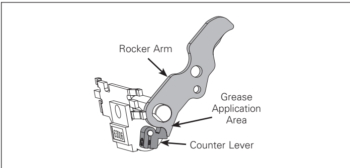
Figure 8. Step 5
