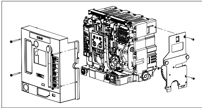
Figure 4. Details for Steps 1 and 2
