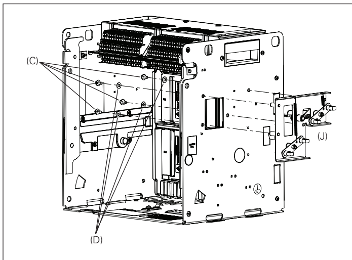
Figure 8. Details for Step 5
