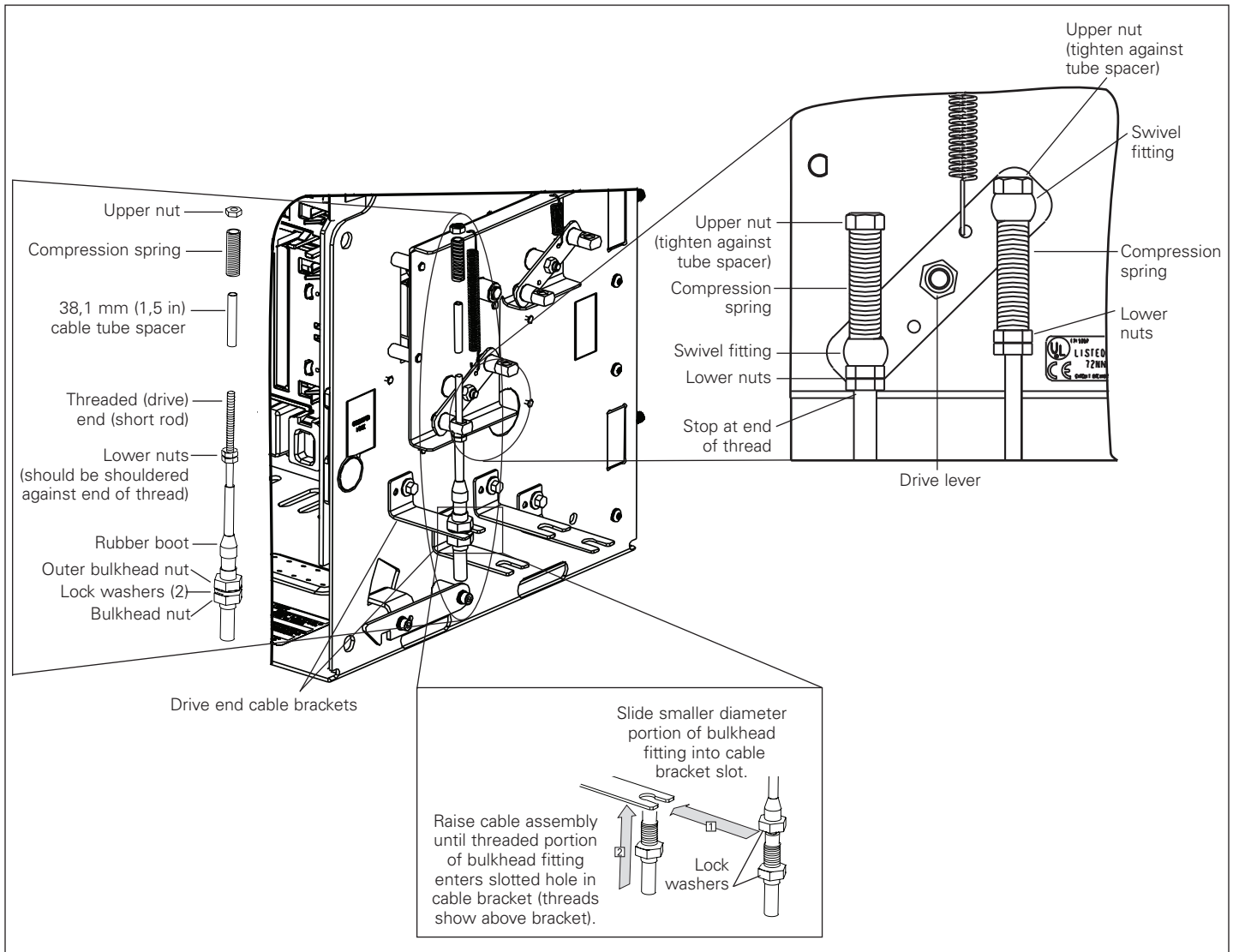
Figure 13. Details for Step 8: Cable assembly drive (short rod) end mounting component identification, mounting cable assembly in cable bracket, and cable rod attachment to drive arm
