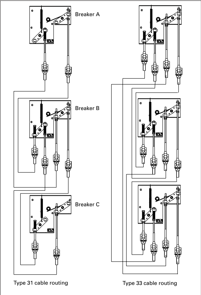
Figure 11. Cable routing for Type 31 and 33 interlock configurations
