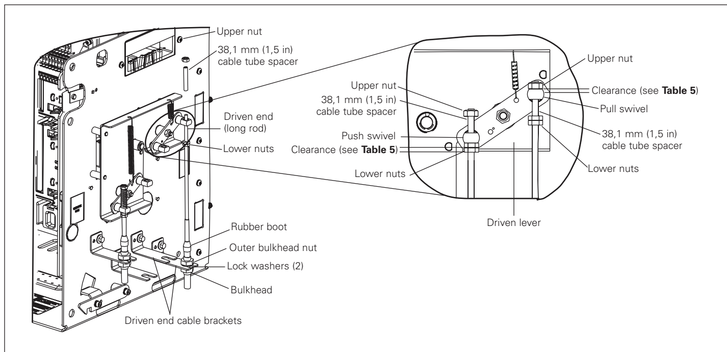
Figure 14. Details for Step 9: driven (long rod) end mounting component identification and Step 10 driven (long rod) end after adjustments
