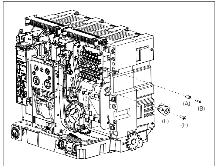
Figure 6. Details for Step 3 and 4
