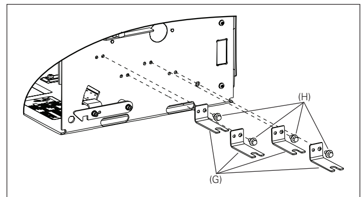
Figure 10. Details for Step 6
