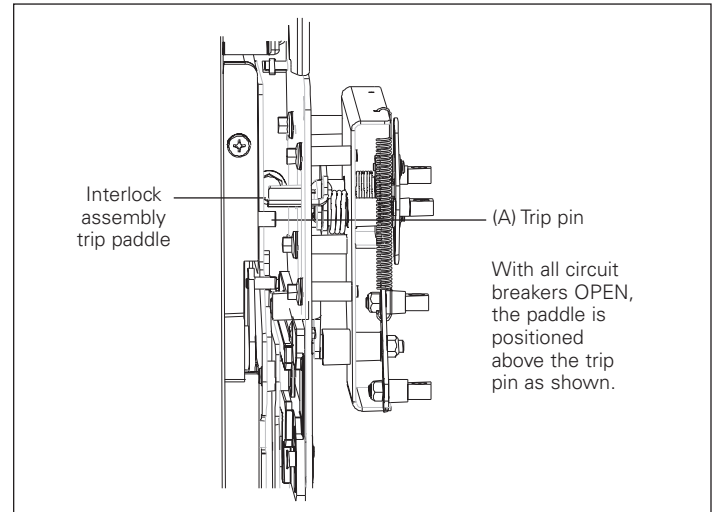
Figure 9. Details for Step 5
