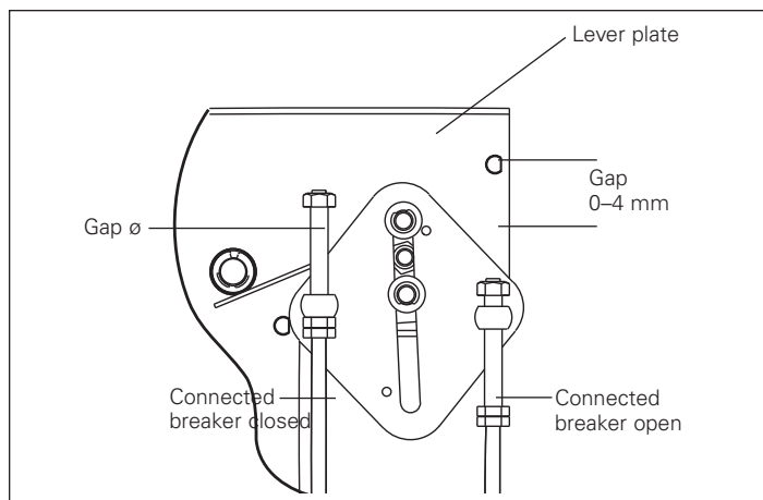
Figure 15. Driven "And" lever position with interconnected push breaker closed and pull breaker open
