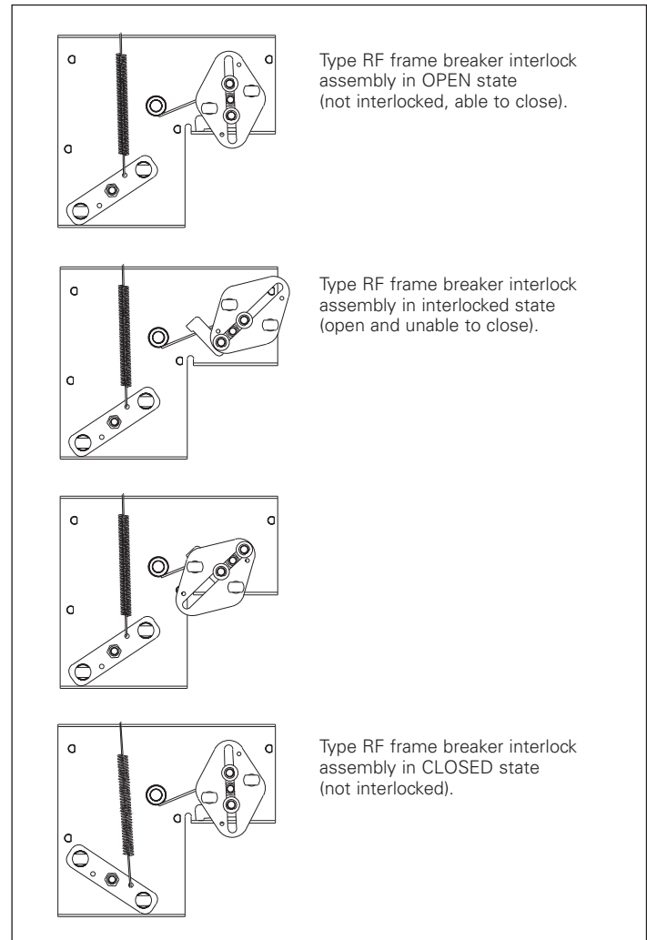
Figure 18. Position of interlock based on breaker state
