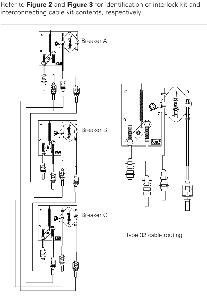
Figure 1. Cable routing for three-way Type 32 interlock configurations
