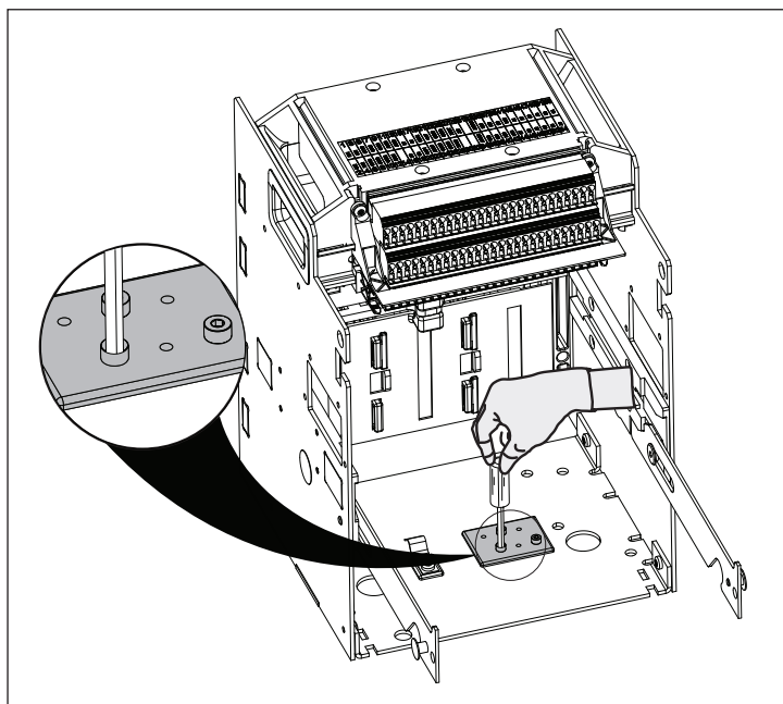
Figure 4. Typical cassette interlock pin location reference.
