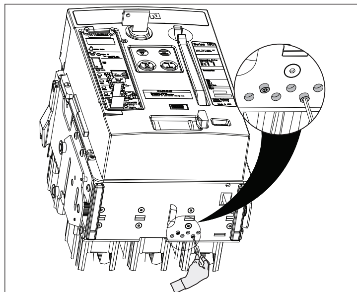
Figure 1. Typical breaker interlock pin location reference.
