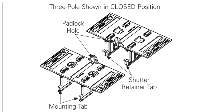
Figure 2. Shutter Assemblies
