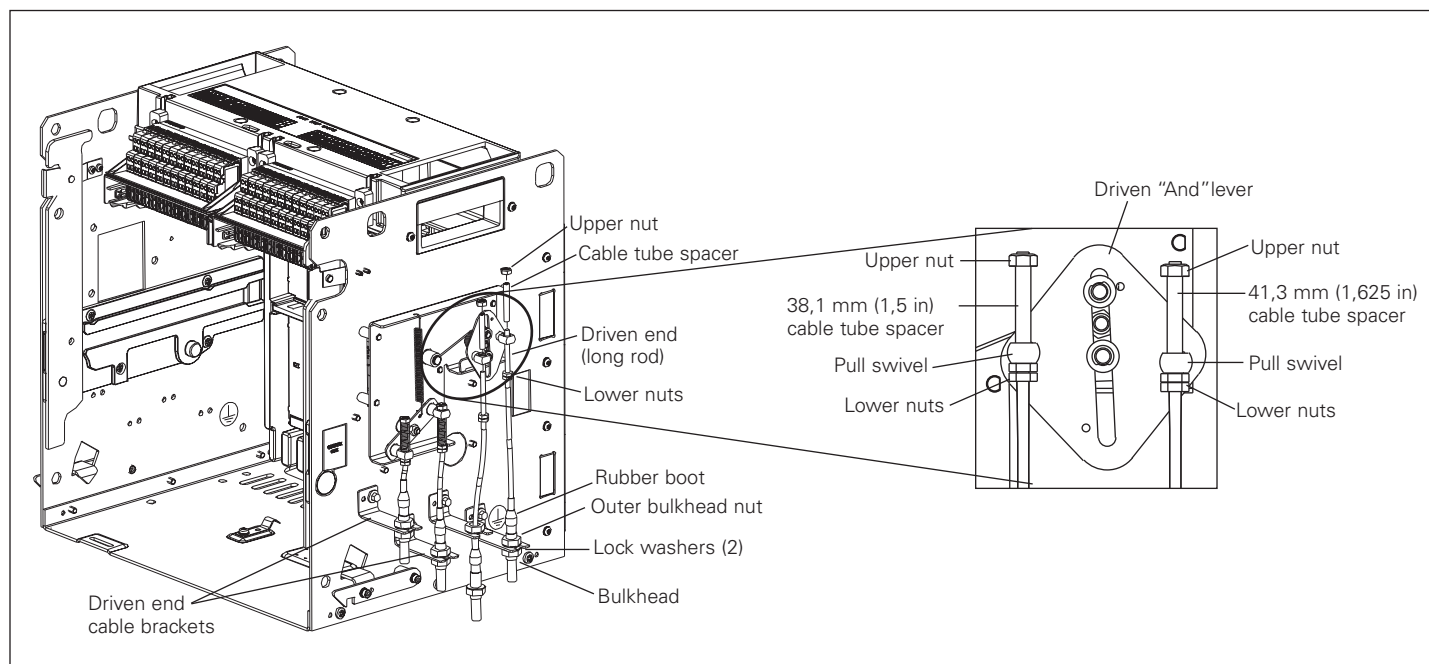
Figure 18. Details for Step 9: driven (long rod) end mounting component identification and Step 10 driven (long rod) end after adjustments
