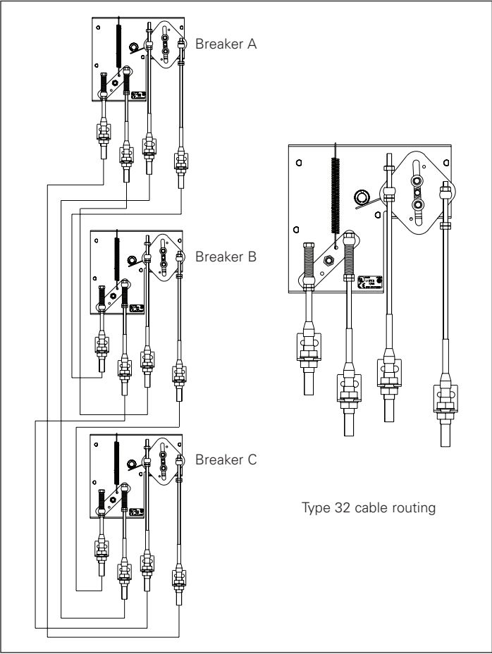
Figure 11. Cable routing for three-way Type 32 interlock configurations
