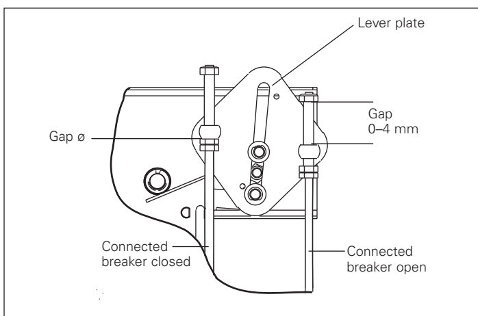
Figure 16. Driven "And" lever position with interconnected push breaker closed and pull breaker open
