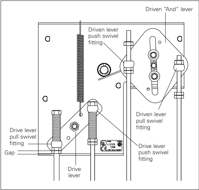
Figure 12. Push and pull swivel fitting identification
