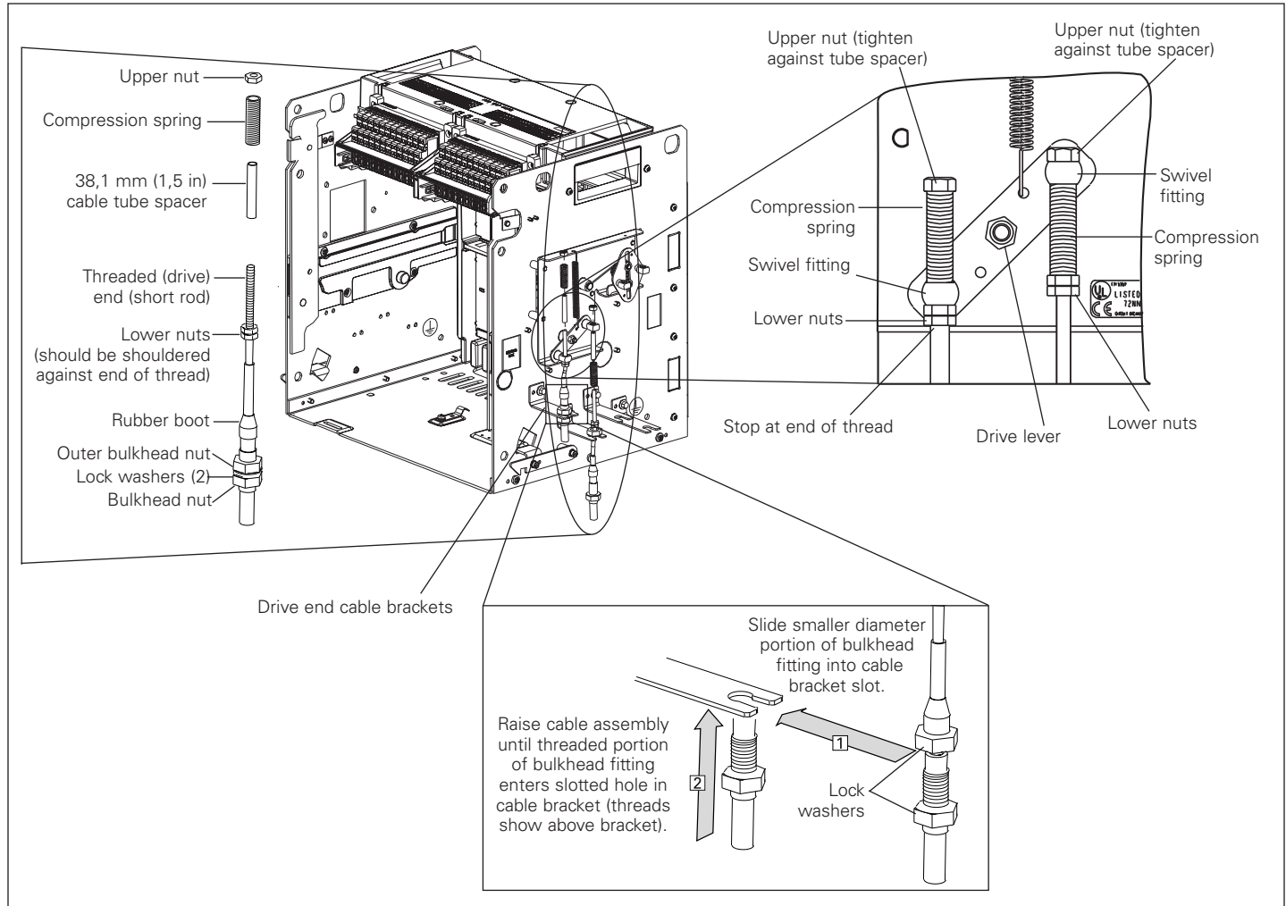
Figure 13. Details for Step 8: cable assembly drive (short rod) end mounting component identification, mounting cable assembly in cable bracket, and cable rod attachment to drive arm
