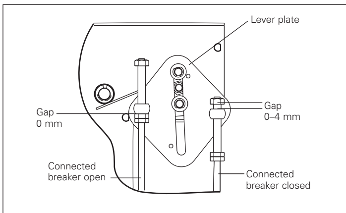
Figure 15. Driven "And" lever position with interconnected push breaker open and pull breaker closed
