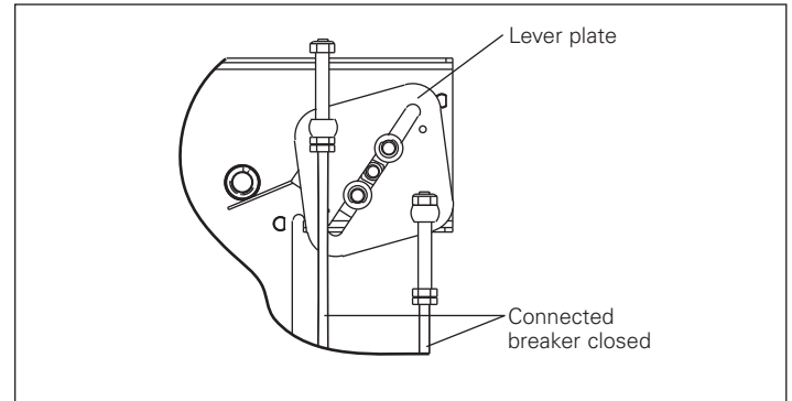
Figure 17. Driven "And" lever position with interconnected breakers closed
