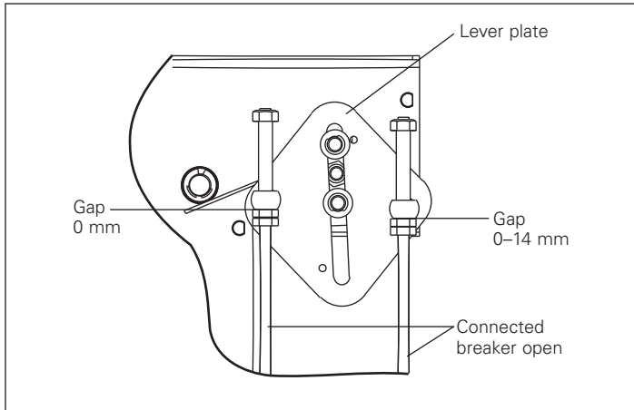
Figure 14. Driven "And" lever position with interconnected breakers open
