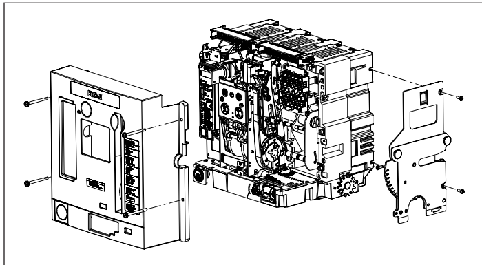
Figure 4. Details for Steps 1 and 2
