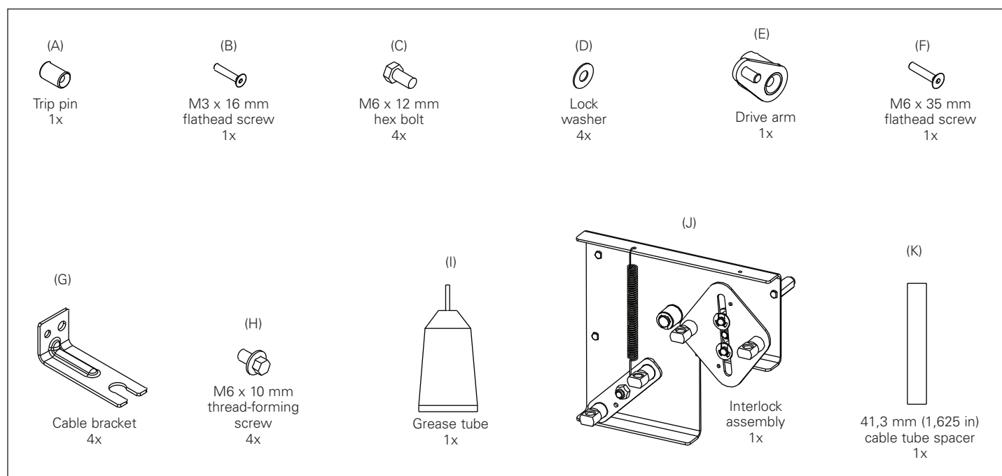
Figure 2. Interlock kit part identification, includes parts to install on a single drawout Type RF frame breaker and cassette (does not include cables)
