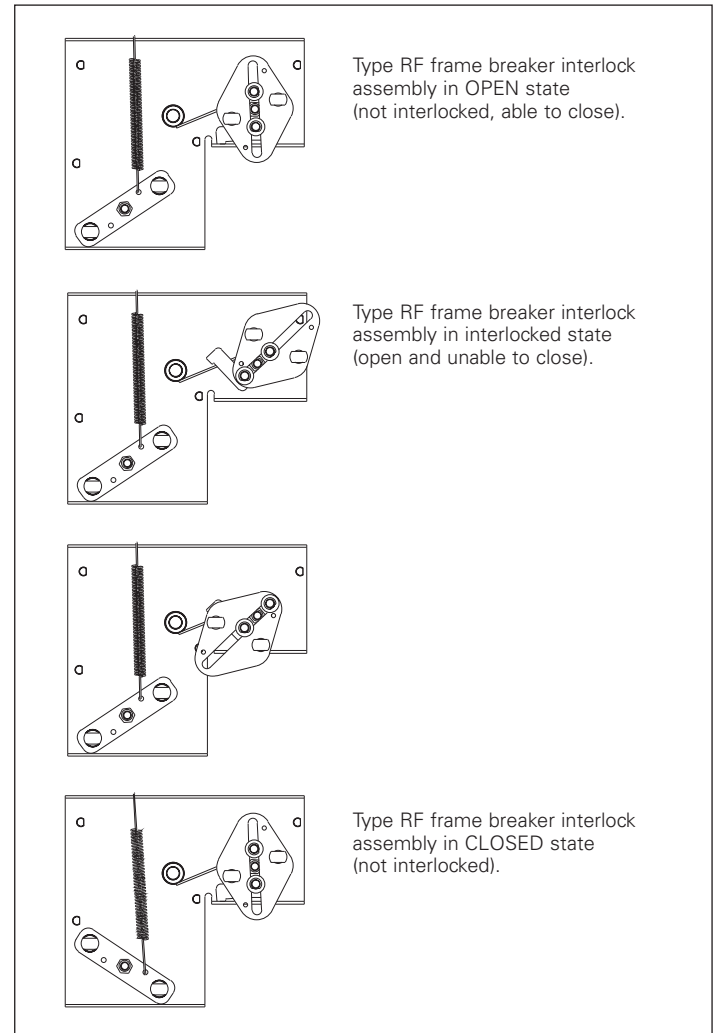
Figure 19. Position of interlock based on breaker state
