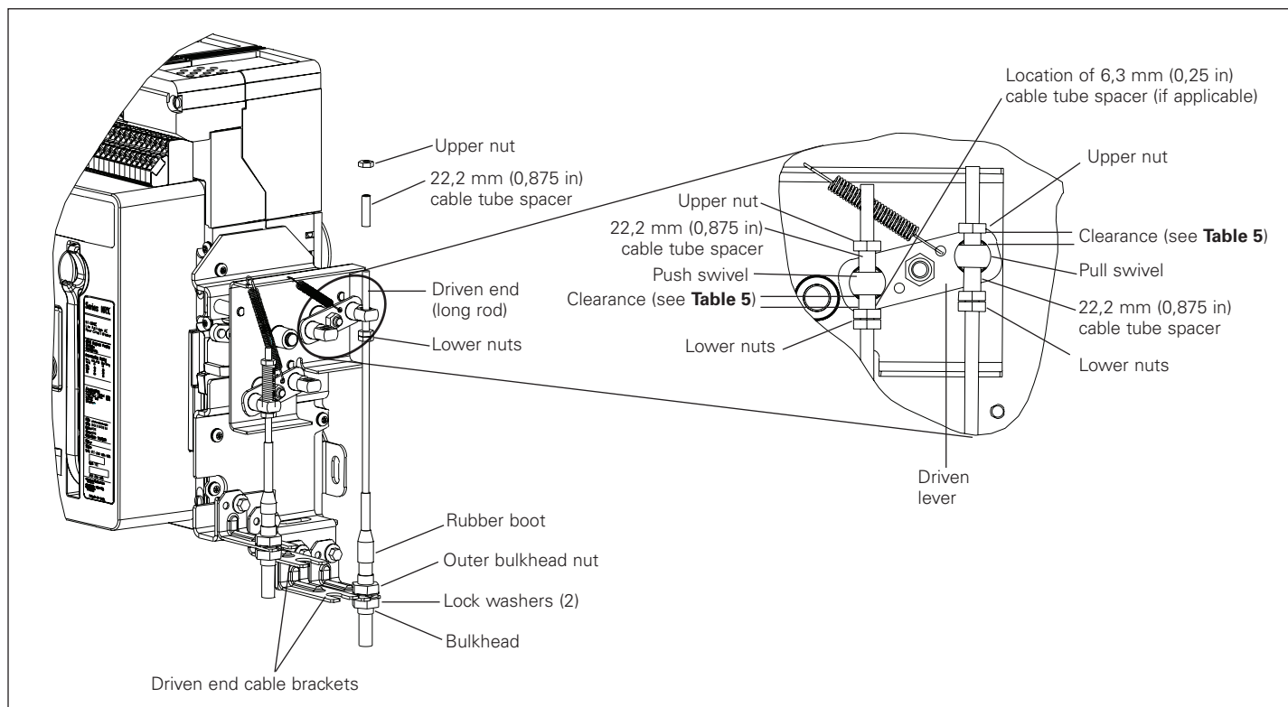
Figure 14. Details for Step 11: driven (long rod) end mounting component identification and Step 12 driven (long rod) end after adjustments
