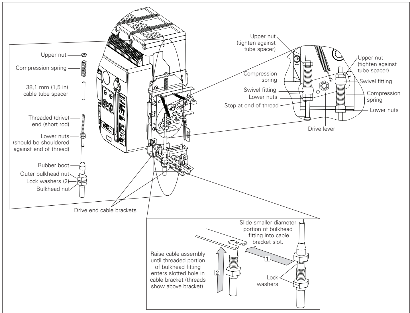
Figure 13. Details for Step 10: cable assembly drive (short rod) end mounting component identification, mounting cable assembly in cable bracket, and cable rod attachment to drive arm
