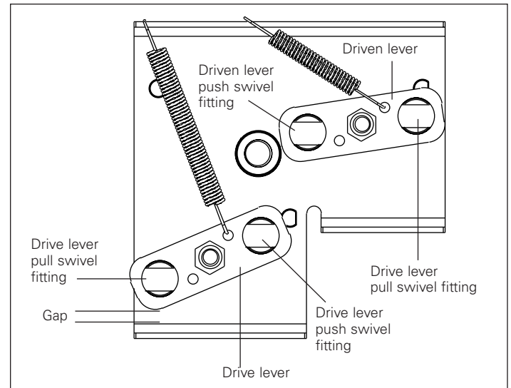
Figure 12. Push and pull swivel fitting identification
