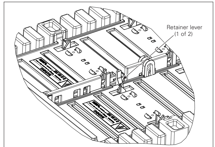
Figure 6. Retainer tabs.
