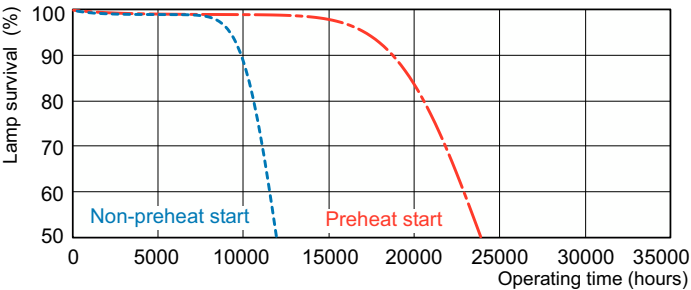
Life Expectancy Diagram - MASTER TL5 HE 14W/830 1SL/20
