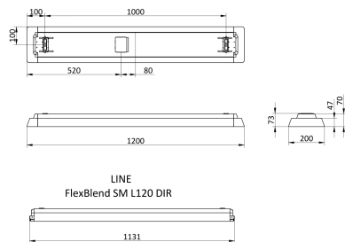
FlexBlend SM L120 DIR
